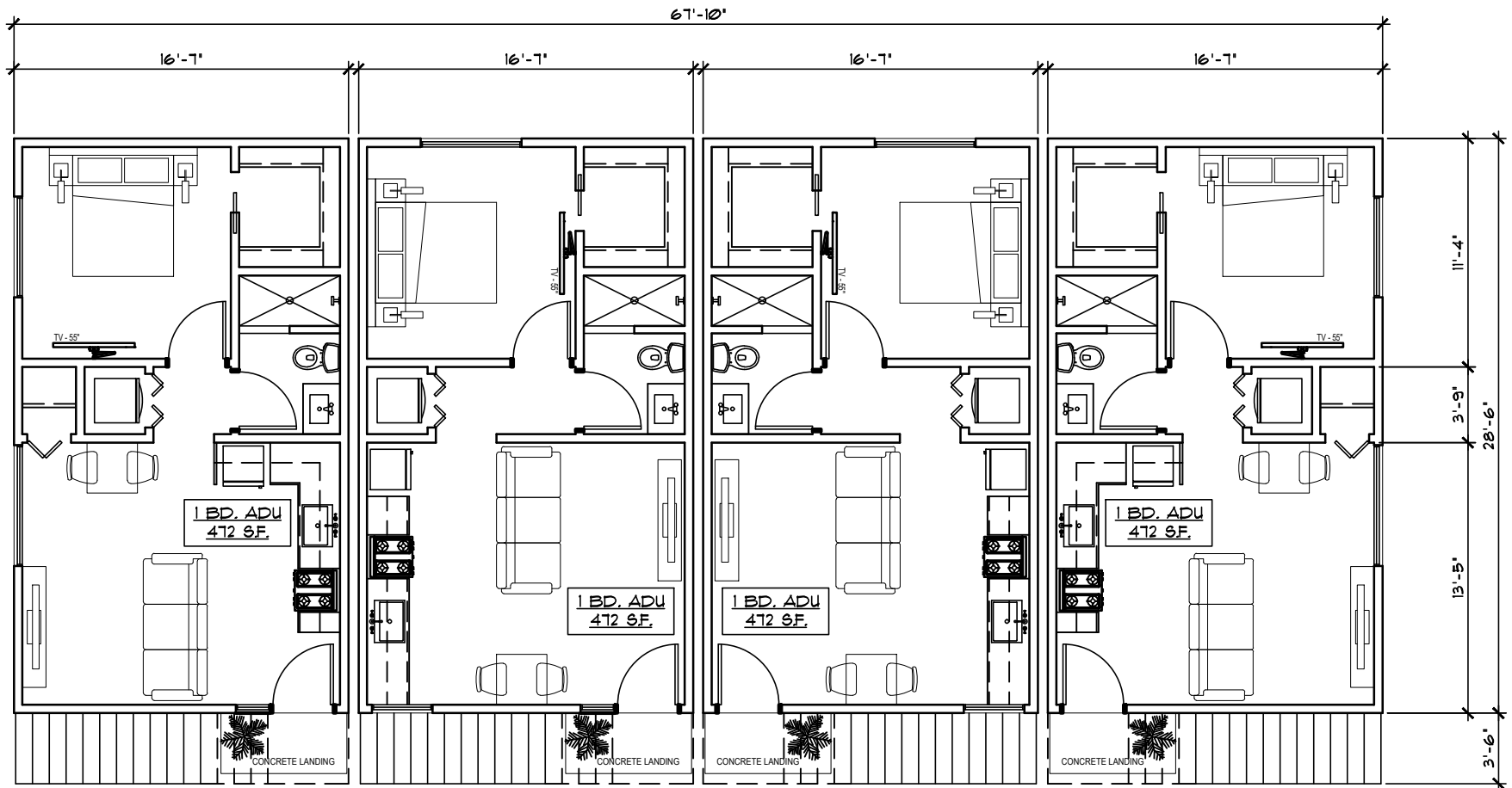
FLOOR PLAN 1ST FLOOR
